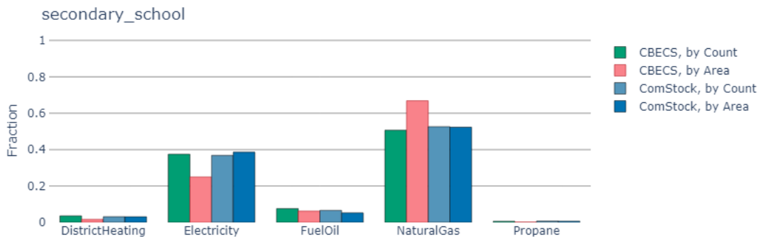
Figure 71. Area-weighted vs. building-count-weighted comparison of fuel type prevalence between ComStock and CBECS for secondary schools. From left to right, the fuel types on the x-axis are: district heating, electricity, fuel oil, natural gas, and propane.
