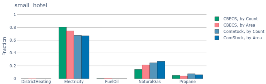
Figure 72. Area-weighted vs. building-count-weighted comparison of fuel type prevalence between ComStock and CBECS for small hotel. From left to right, the fuel types on the x-axis are: district heating, electricity, fuel oil, natural gas, and propane.
