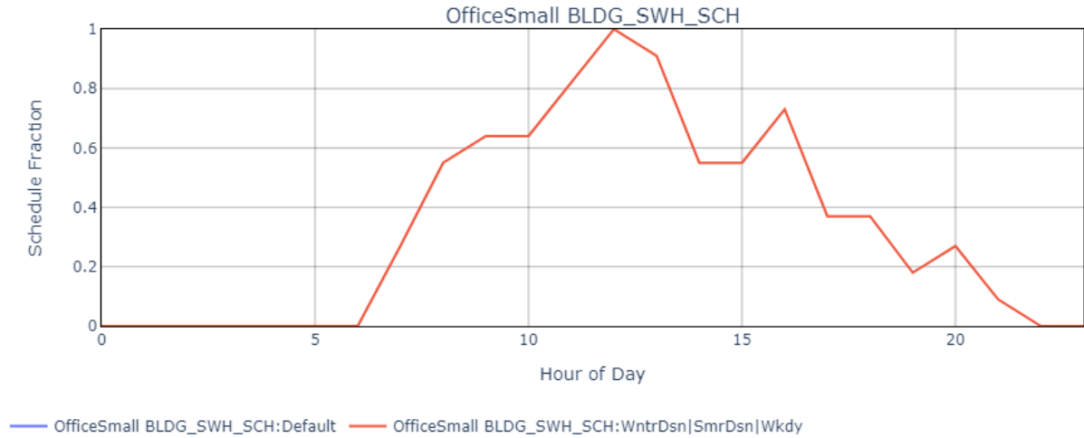
Figure 54. SWH heating usage schedule for small offices.
