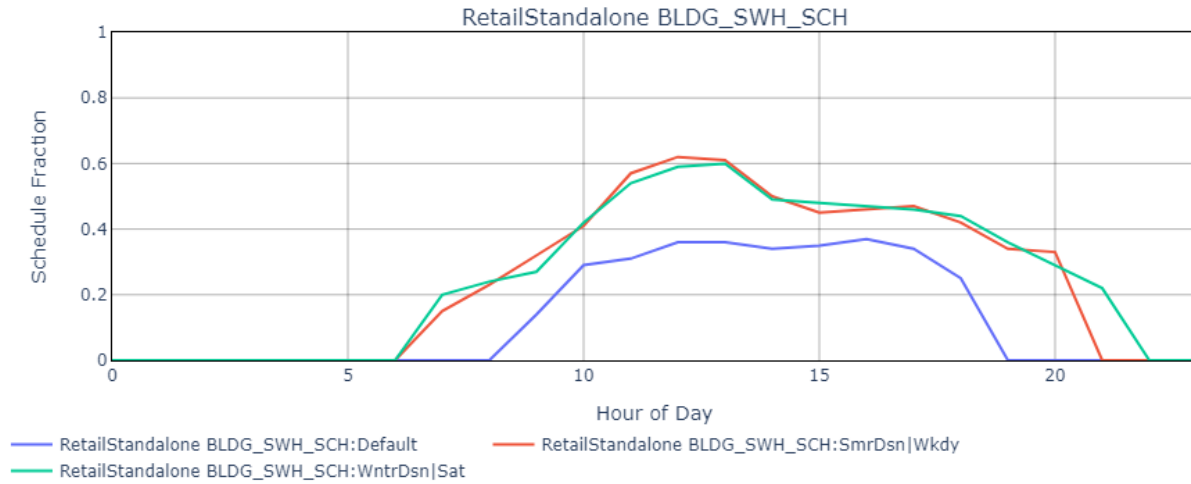
Figure 58. SWH heating usage schedule for retail.
