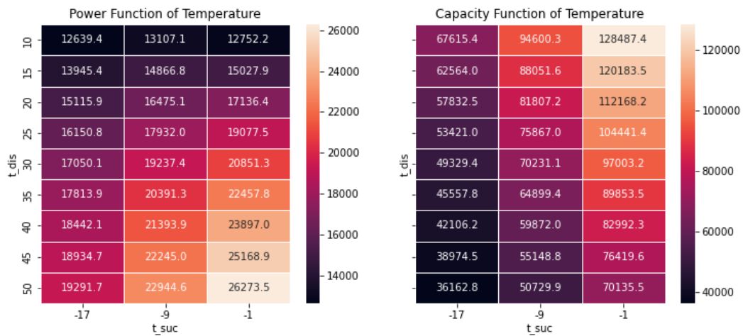
Figure 111. Power and capacity values as a function of suction and discharge temperature for large, new, medium-temperature compressors.
