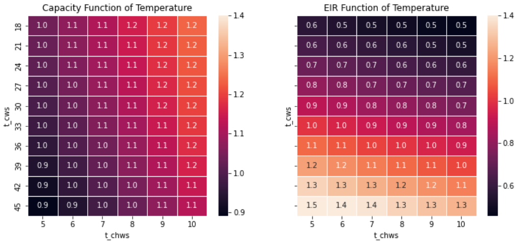
Figure 107. Performance curves for "WaterCooled PositiveDisplacement Chiller LT150 2010 Modifiers" WCC.
