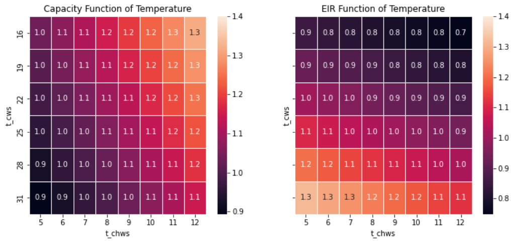
Figure 108. Performance curves for “ChlrWtrPosDispPathAAll Modifiers” WCC.
