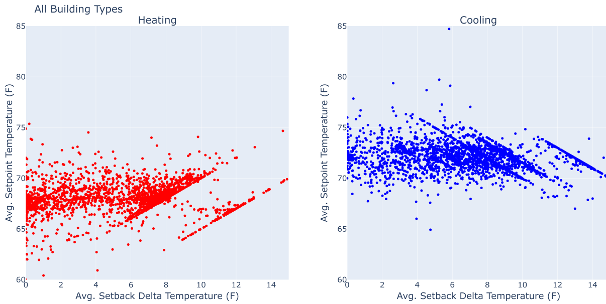
Figure 91. Thermostat heating and cooling set point-setback delta correlation from BAS data sources; all building types.
