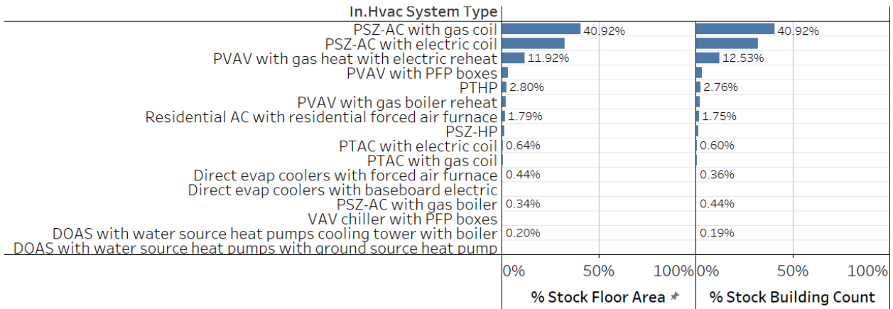
Figure 84. Prevalence of ComStock HVAC system types by total stock floor area and building count; strip malls.
