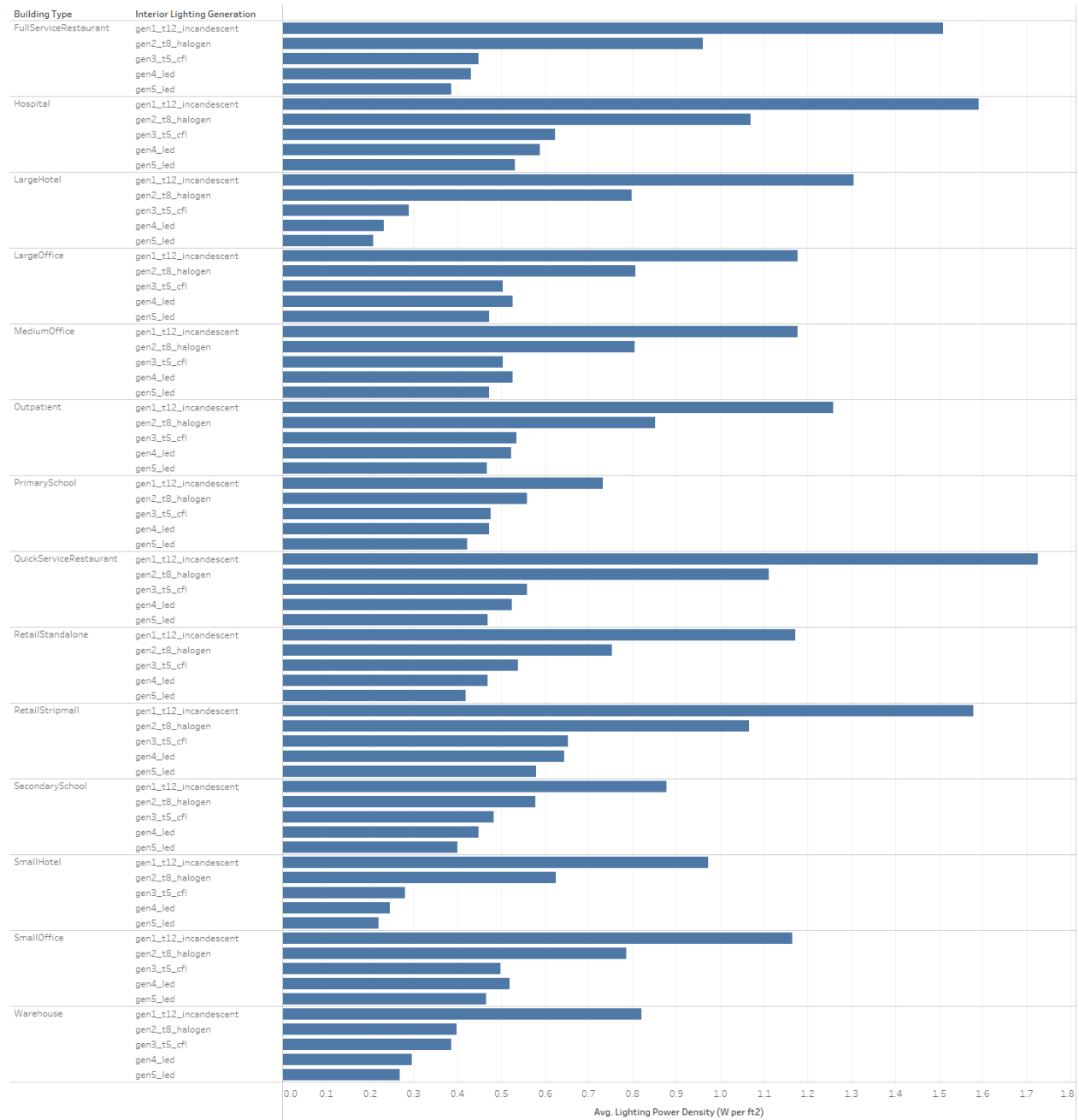
Figure 25. Average interior lighting power density by building type and lighting generation.
