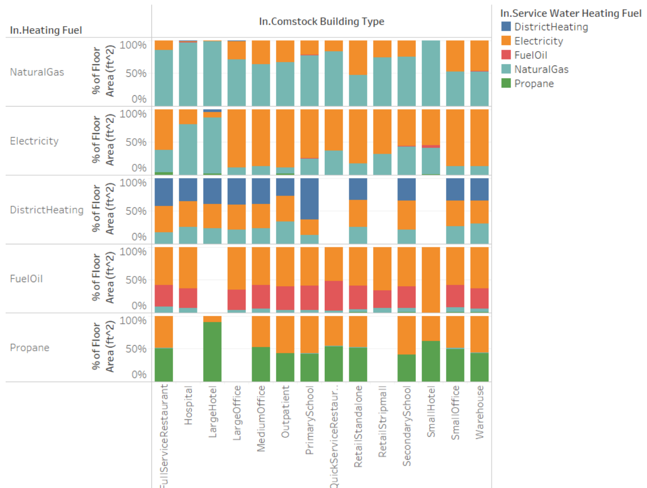
Figure 32. Area-weighted distribution of service water heating fuel by space heating fuel and building type.
