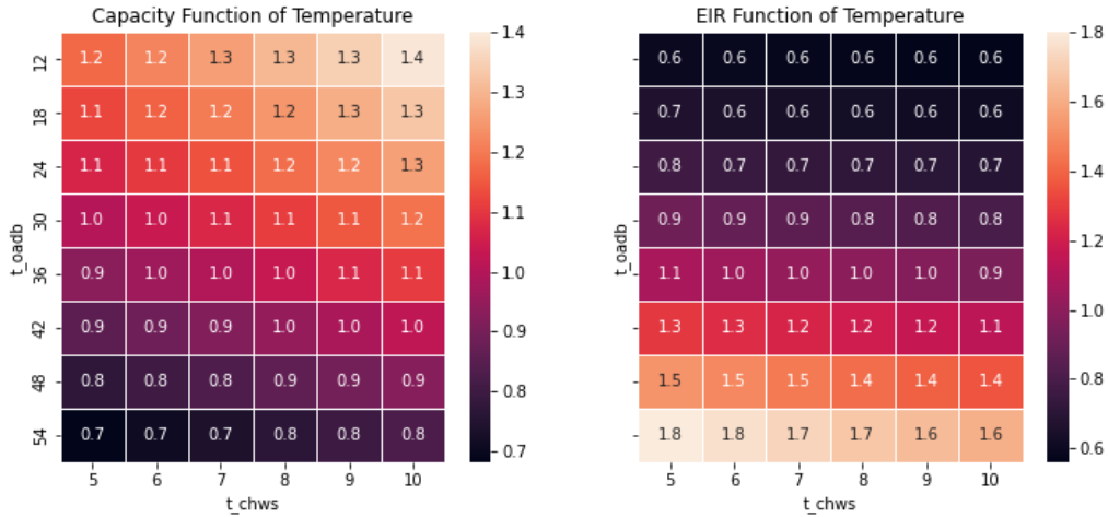
Figure 104. “AirCooledChiller2010PathA” modifier performance curves; capacity as a function of temperature and EIR as a function of temperature. Independent variables beyond the curve limits will use the bound of the curve limit during simulation.
