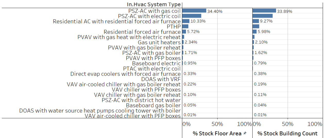
Figure 89. Prevalence of ComStock HVAC system types by total stock floor area and building count; warehouses.
