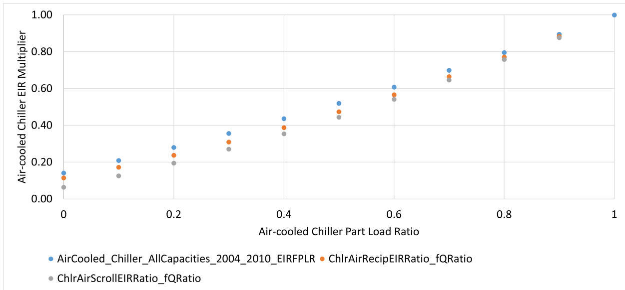
Figure 103. Air-cooled chiller EIR as a function of part load ratio performance curves. Independent variables beyond the curve limits will use the bound of the curve limit during simulation.
