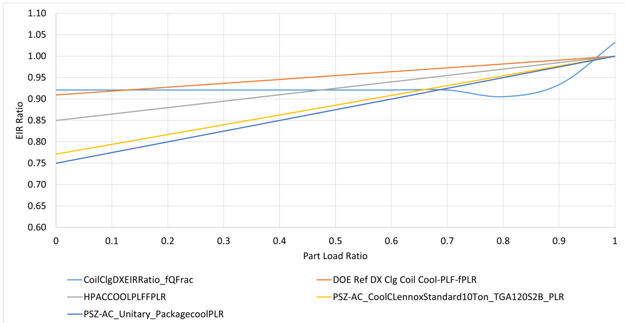
Figure 93. DX cooling energy input ratio as a function of part load ratio performance curves.
