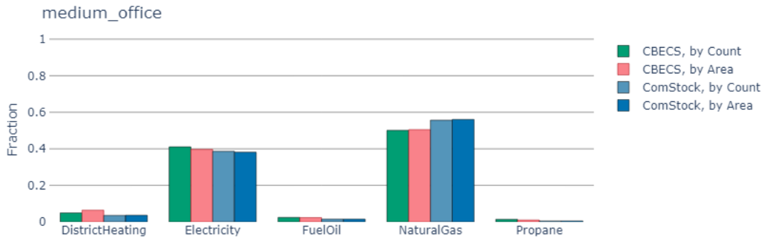
Figure 66. Area-weighted vs. building-count-weighted comparison of fuel type prevalence between ComStock and CBECS for medium offices. From left to right, the fuel types on the x-axis are: district heating, electricity, fuel oil, natural gas, and propane.
