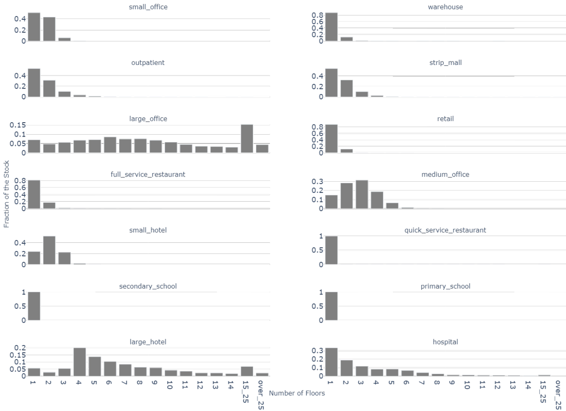
Figure 15. Distribution of number of aboveground floors by building type. The x-axis represents the number of floors, and the y-axis represents the fraction of the building stock.
