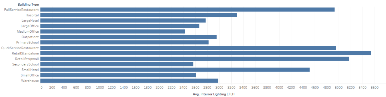
Figure 30. Average interior lighting equivalent full load hours by building type.
