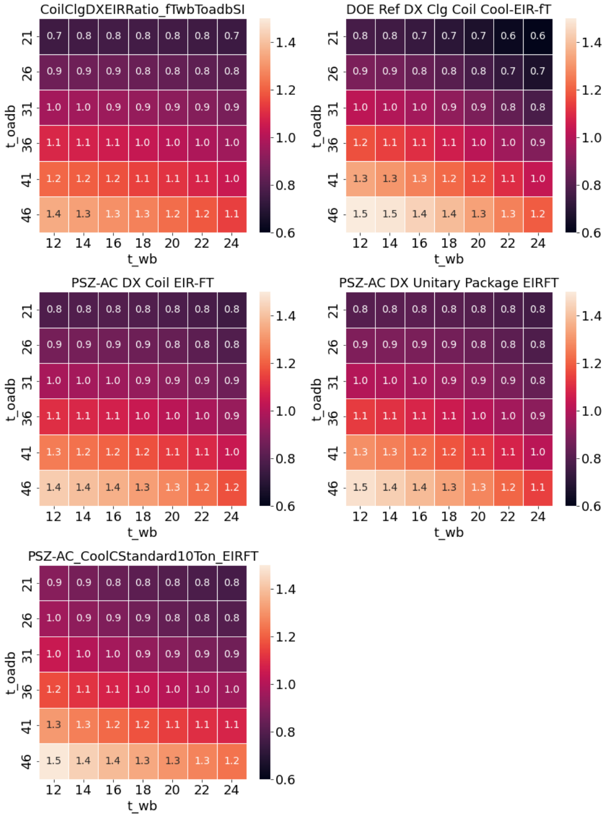
Figure 96. DX cooling energy input ratio as a function of temperature performance curves. Independent variables are outdoor air dry bulb temperature (y-axis, degrees Celsius) and wet bulb temperature entering the cooling coil (x-axis, degrees Celsius).
