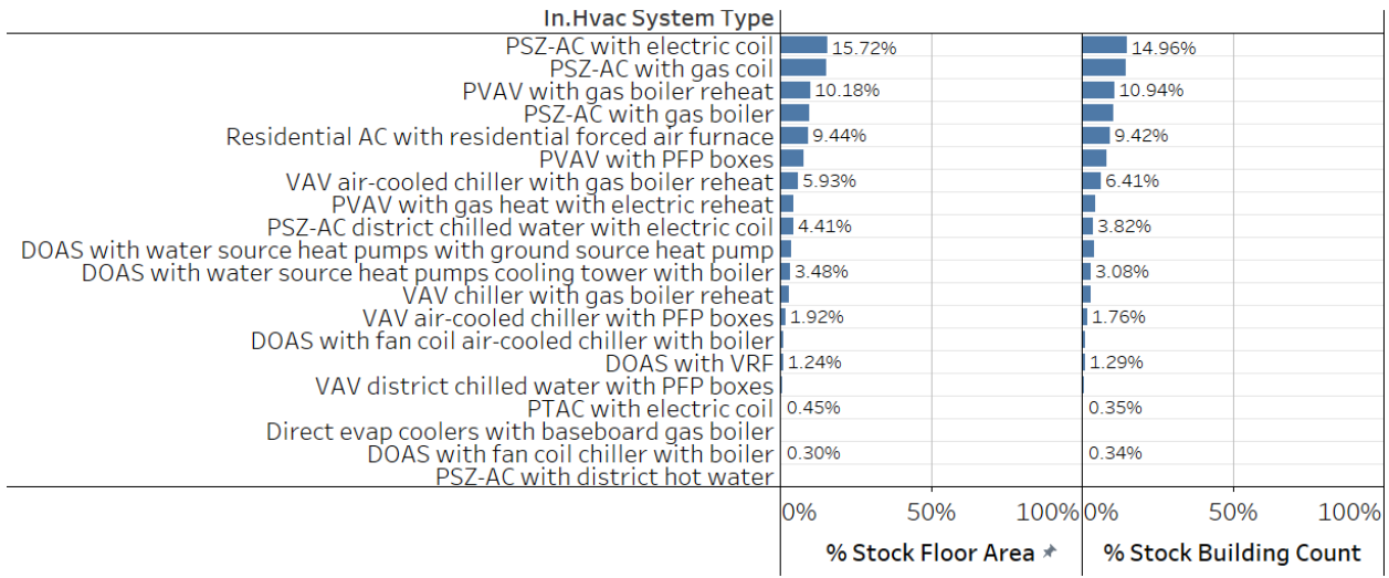
Figure 82. Prevalence of ComStock HVAC system types by total stock floor area and building count; primary schools.
