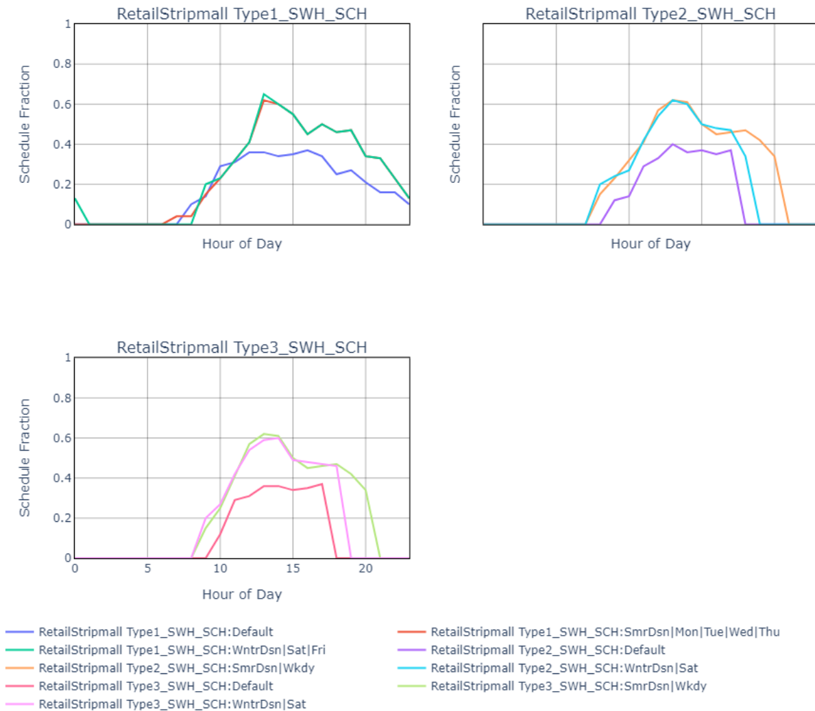
Figure 61. SWH heating usage schedule for strip mall.
