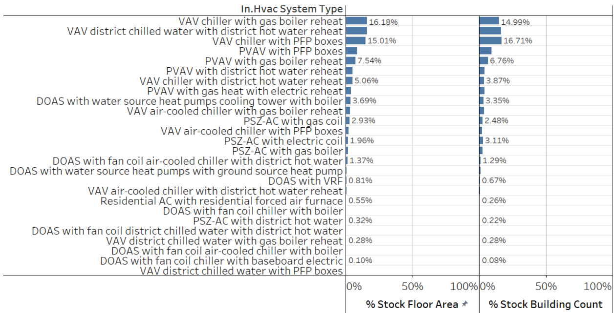
Figure 79. Prevalence of ComStock HVAC system types by total stock floor area and building count; large offices.
