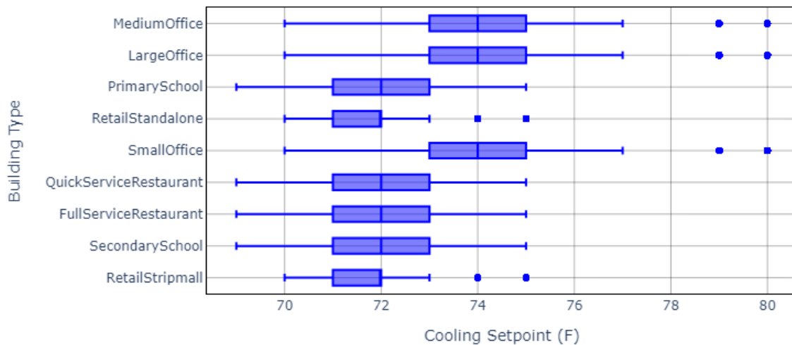
Figure 40. Cooling thermostat set point (Fahrenheit) distributions per building type.
