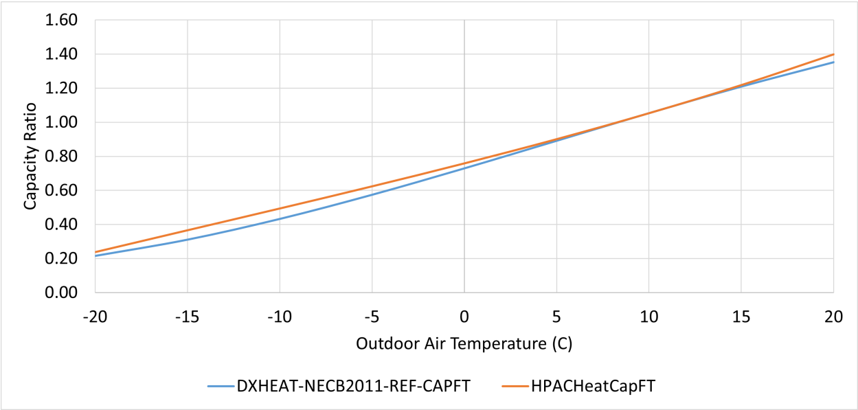
Figure 101. Air-source heat pump capacity as a function of outdoor air dry bulb temperature.
