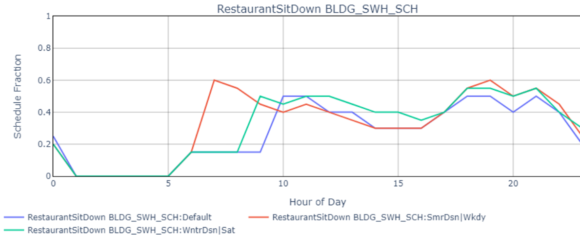
Figure 49. SWH heating usage schedule for full service restaurants.
