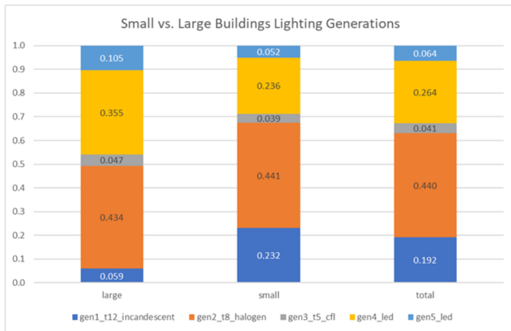
Figure 27. Fraction of installed lighting generations by building size (count-based distribution).
