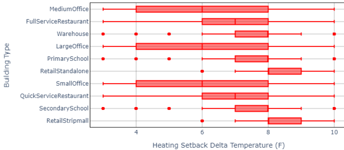
Figure 41. Thermostat heating setback delta temperature probability distributions per building type.
