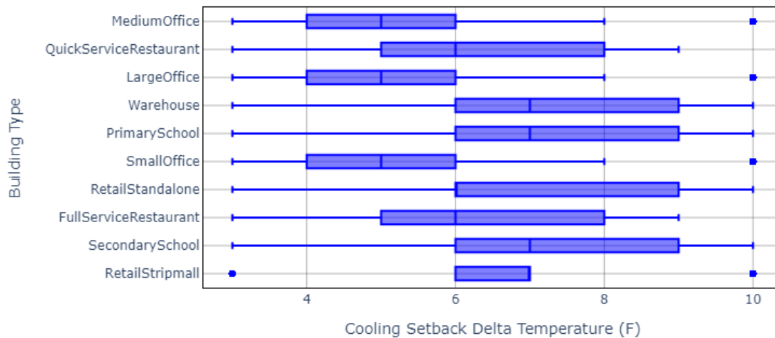
Figure 42. Thermostat cooling setback delta temperature probability distributions per building type.
