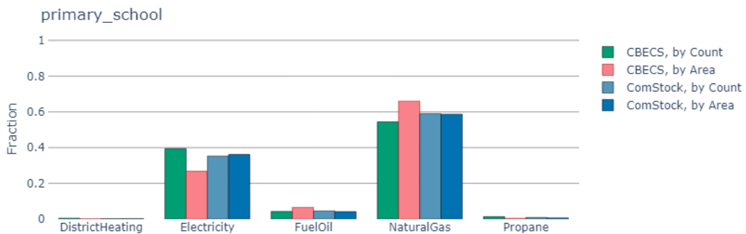
Figure 68. Area-weighted vs. building-count-weighted comparison of fuel type prevalence between ComStock and CBECS for primary schools. From left to right, the fuel types on the x-axis are: district heating, electricity, fuel oil, natural gas, and propane.
