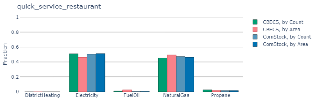
Figure 69. Area-weighted vs. building-count-weighted comparison of fuel type prevalence between ComStock and CBECS for quick service restaurants. From left to right, the fuel types on the x-axis are: district heating, electricity, fuel oil, natural gas, and propane.
