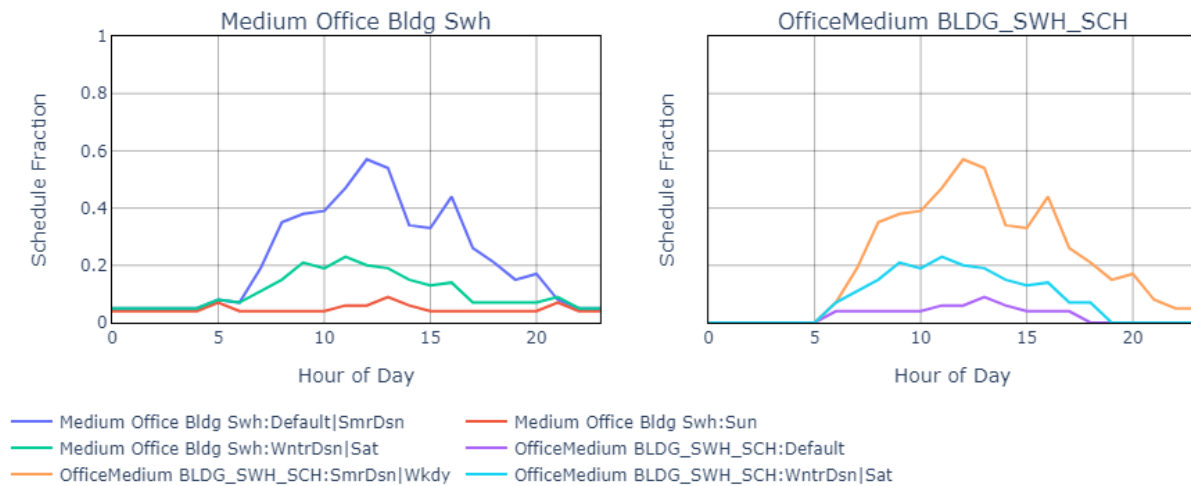
Figure 53. SWH heating usage schedule for medium office.
