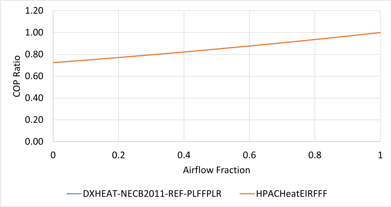
Figure 100. Air-source heat pump EIR ratio as a function of airflow fraction.
