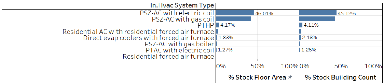
Figure 83. Prevalence of ComStock HVAC system types by total stock floor area and building count; quick service restaurants.
