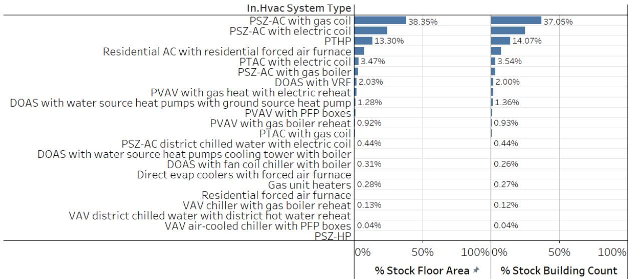
Figure 88. Prevalence of ComStock HVAC system types by total stock floor area and building count; small offices.
