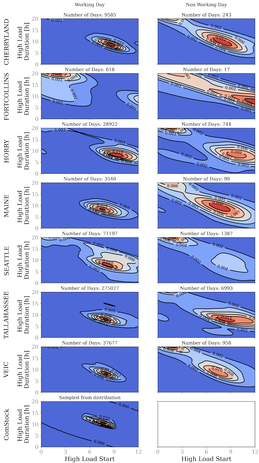
Figure 46. Distribution of small office hours of operations extracted from AMI data (from seven utilities), by utility and day type, and compared to ComStock before updates. This figure shows how the hours of operation (start time and duration of the high load period) are influenced by utility region (all seasons are combined in this plot).
