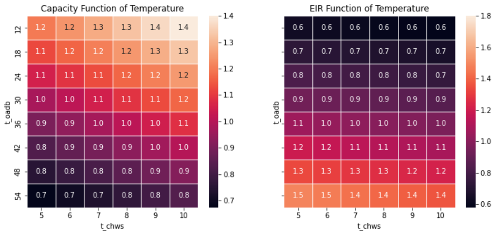
Figure 105. “ChlrAirRecip” modifier performance curves; capacity as a function of temperature and EIR as a function of temperature. Independent variables beyond the curve limits will use the bound of the curve limit during simulation.
