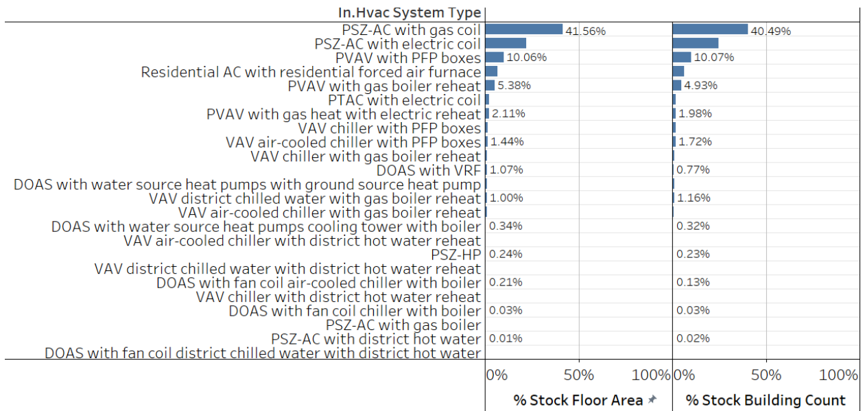
Figure 81. Prevalence of ComStock HVAC system types by total stock floor area and building count; outpatient.
