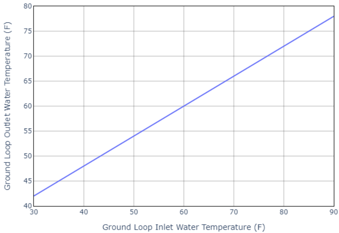
Figure 109. Ground loop outlet vs. inlet temperature relationship for GSHPs.
