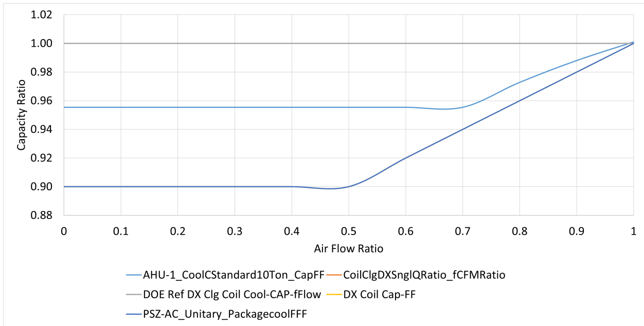
Figure 94. DX cooling capacity as a function of airflow performance curves.
