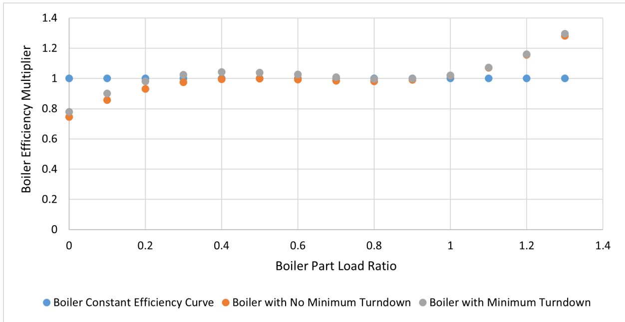
Figure 92. Boiler part load performance curves.
