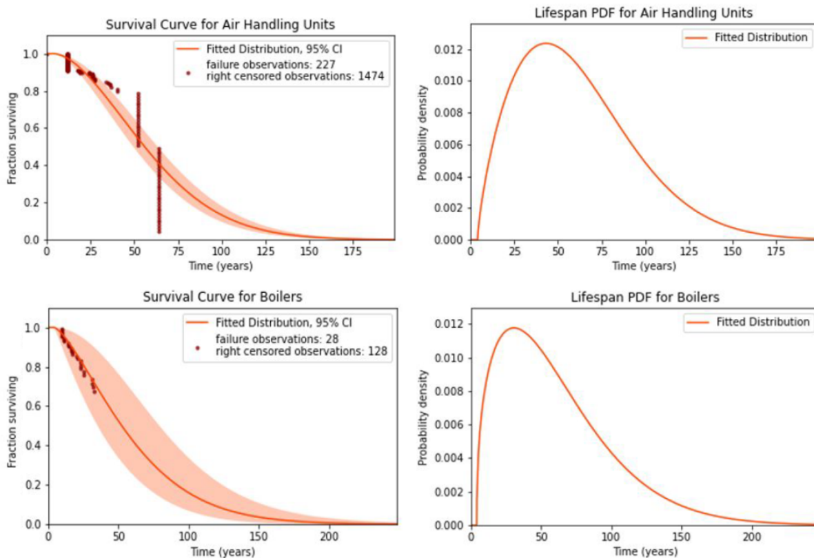
Figure 5. Survival curves and derived lifespan probability density functions for commercial HVAC equipment.
