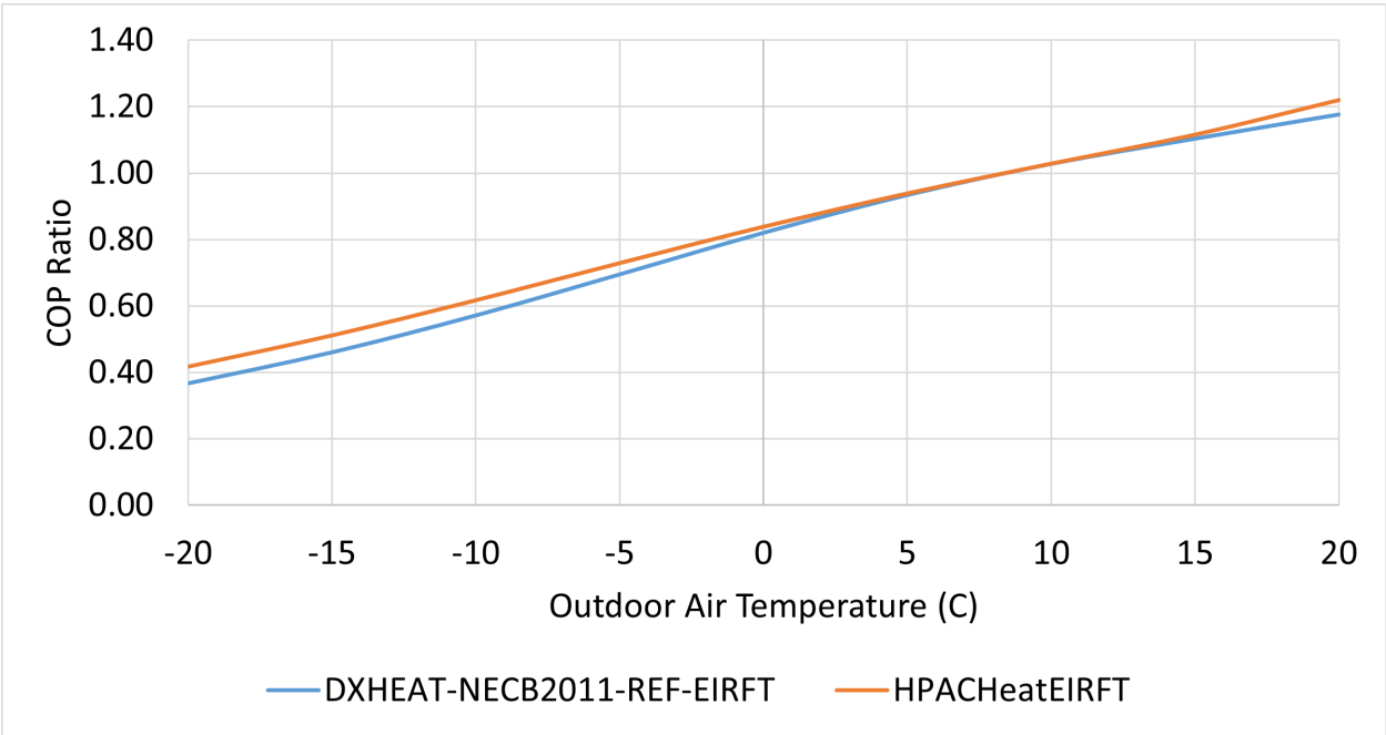
Figure 98. Air-source heat pump COP ratio as a function of outdoor air dry bulb temperature.
