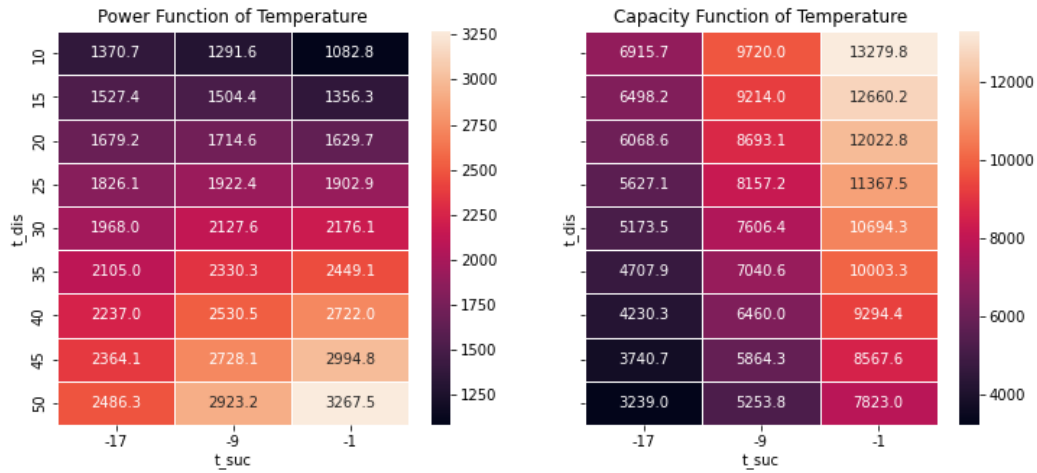
Figure 110. Power and capacity values as a function of suction and discharge temperature for small, old, medium-temperature compressors.
