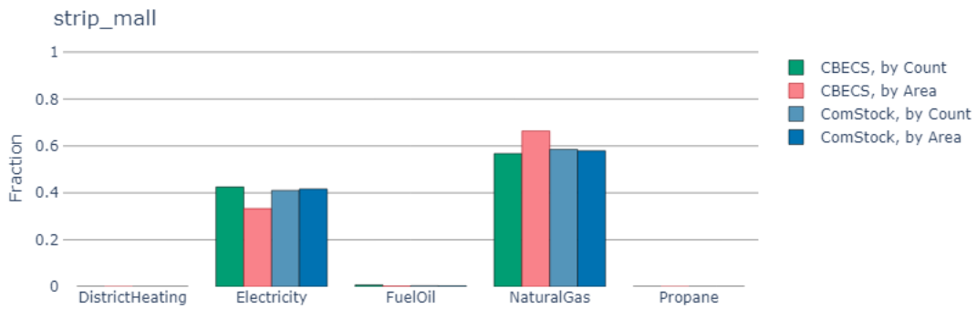
Figure 74. Area-weighted vs. building-count-weighted comparison of fuel type prevalence between ComStock and CBECS for strip malls. From left to right, the fuel types on the x-axis are: district heating, electricity, fuel oil, natural gas, and propane.
