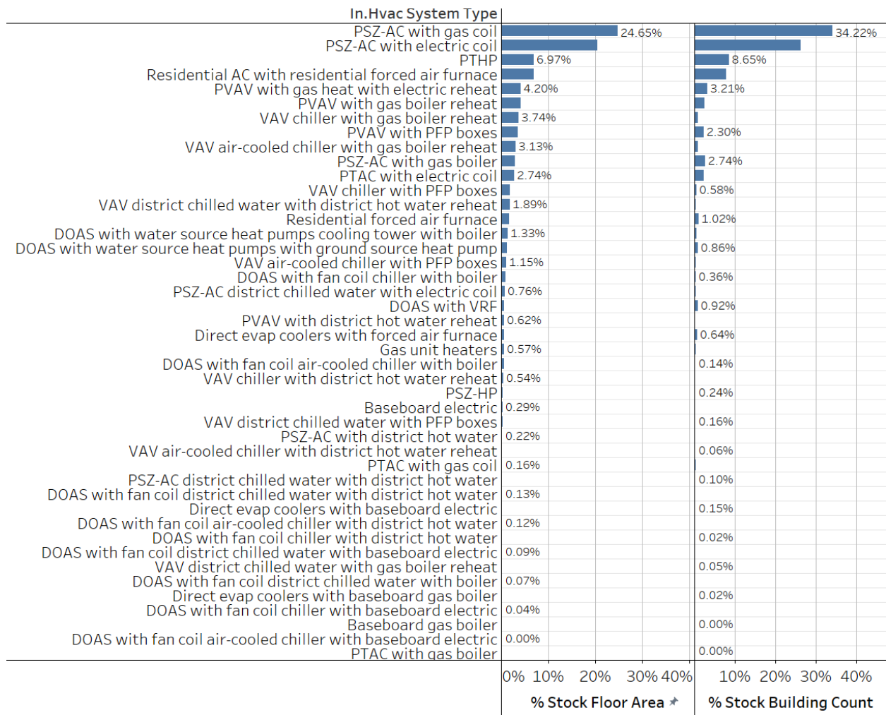
Figure 76. Prevalence of ComStock HVAC system types by total stock floor area and building count; all building types.
