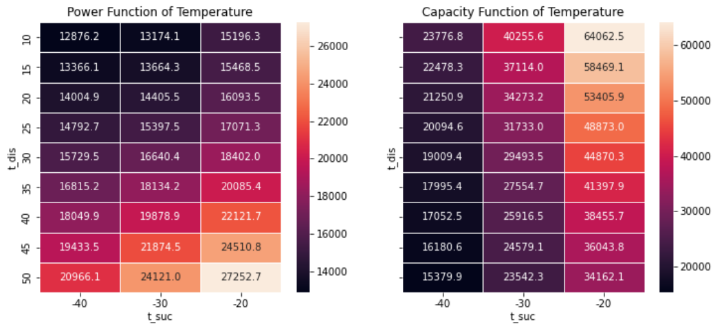
Figure 113. Power and capacity values as a function of suction and discharge temperature for large, new, low-temperature compressors.
