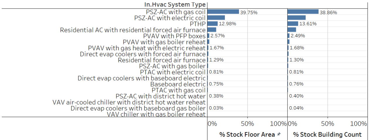
Figure 85. Prevalence of ComStock HVAC system types by total stock floor area and building count; retail.
