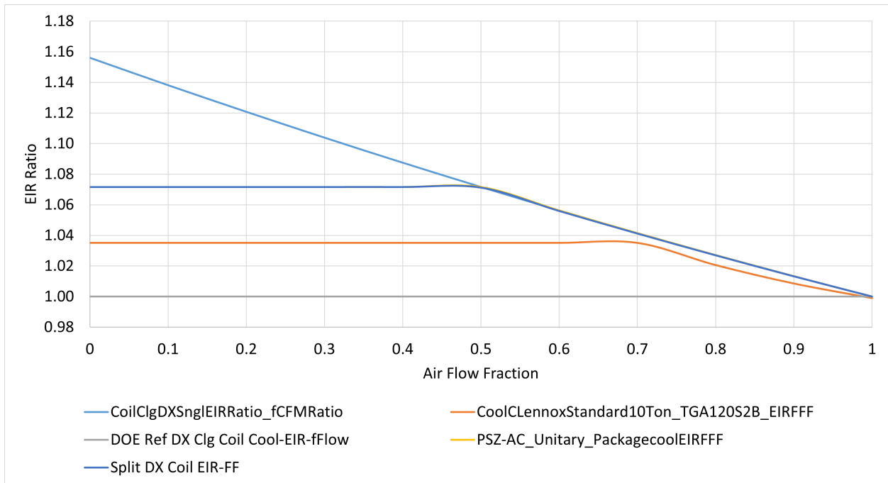
Figure 95. DX cooling energy input ratio as a function of airflow performance curves.
