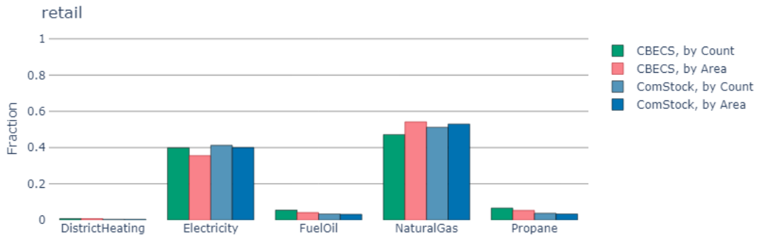
Figure 70. Area-weighted vs. building-count-weighted comparison of fuel type prevalence between ComStock and CBECS for retail. From left to right, the fuel types on the x-axis are: district heating, electricity, fuel oil, natural gas, and propane.
