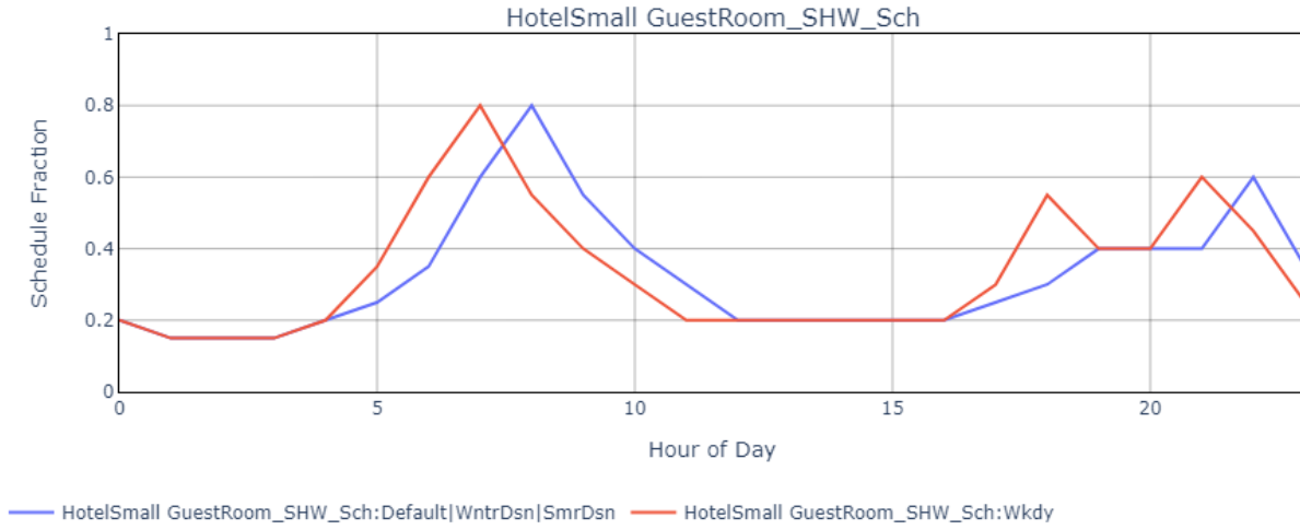
Figure 60. SWH heating usage schedule for small hotel.
