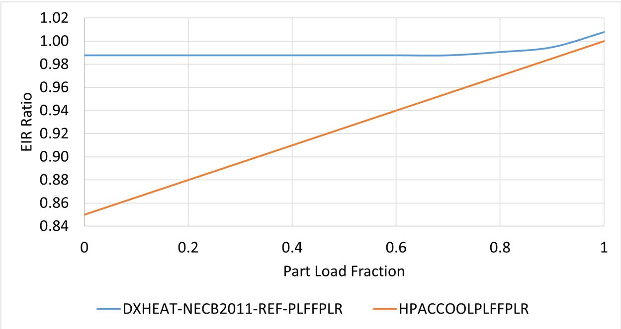
Figure 99. Air-source heat pump EIR ratio as a function of part load ratio.
