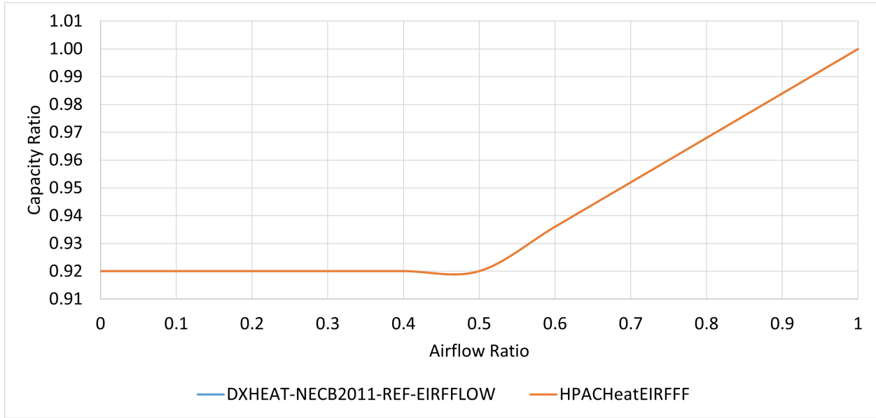
Figure 102. Air-source heat pump capacity as a function of airflow ratio.
