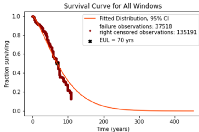
Figure 4. Reliability analysis for windows in commercial buildings, from 2014 CBSA (Navigant Consulting).
