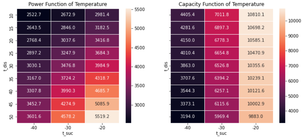
Figure 112. Power and capacity values as a function of suction and discharge temperature for small, old, low-temperature compressors.
