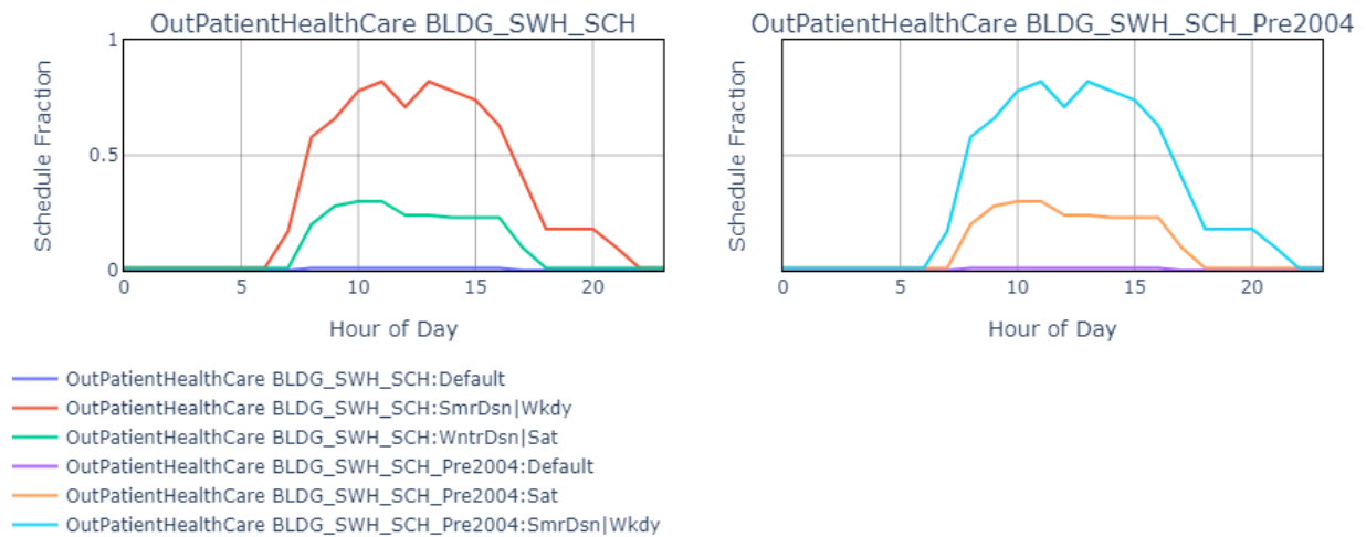
Figure 55. SWH heating usage schedule for outpatient.
