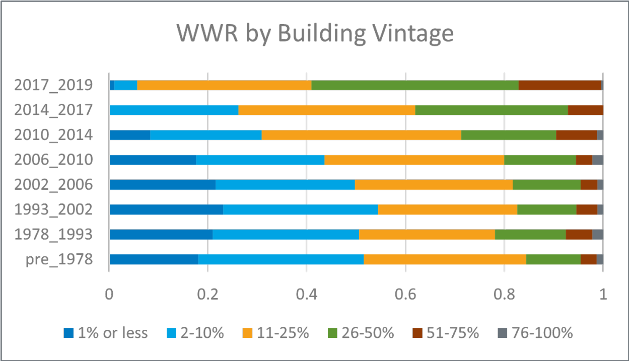
Figure 17. Window-to-wall ratio by building vintage.
