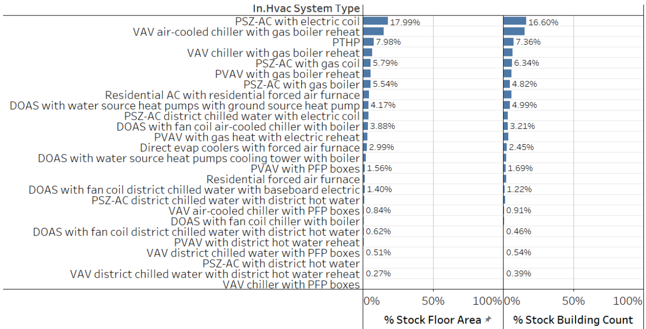
Figure 86. Prevalence of ComStock HVAC system types by total stock floor area and building count; secondary schools.
