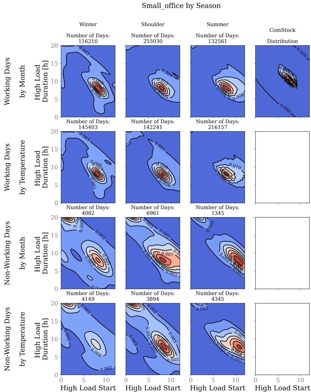
Figure 45. Distribution of small office hours of operations extracted from AMI data (from seven utilities), by day type and season, and compared to ComStock before updates. This figure shows how the hours of operation (start time and duration of the high load period) are influenced by season (all utilities are combined in this plot).
