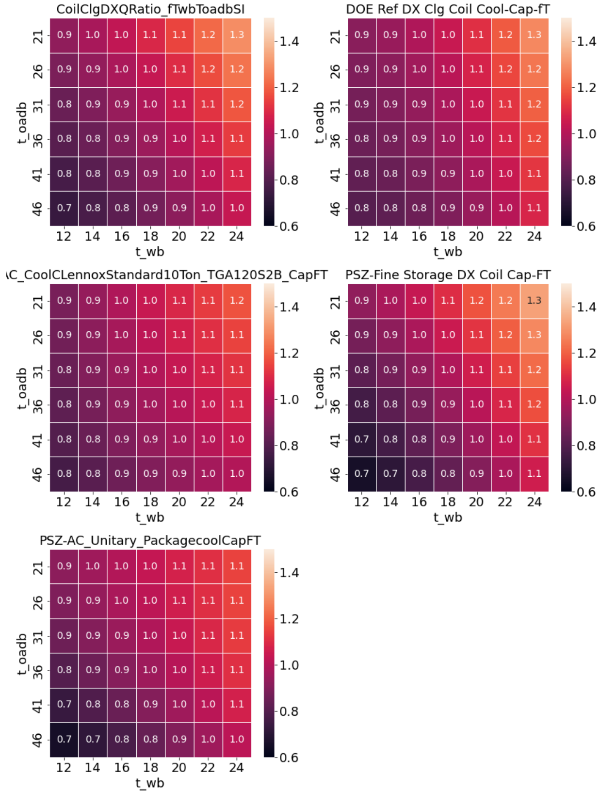
Figure 97. DX cooling capacity as a function of temperature performance curves. Independent variables are outdoor air dry bulb temperature (y-axis, degrees Celsius) and wet bulb temperature entering the cooling coil (x-axis, degrees Celsius).
