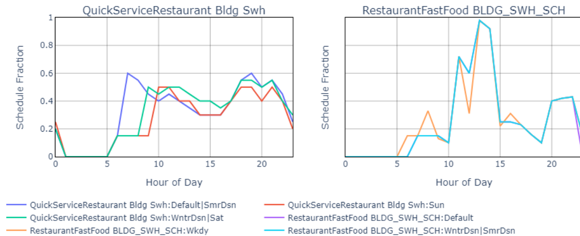
Figure 57. SWH heating usage schedule for quick service restaurant.
