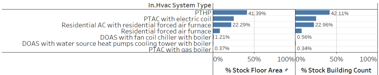
Figure 87. Prevalence of ComStock HVAC system types by total stock floor area and building count; small hotels.
