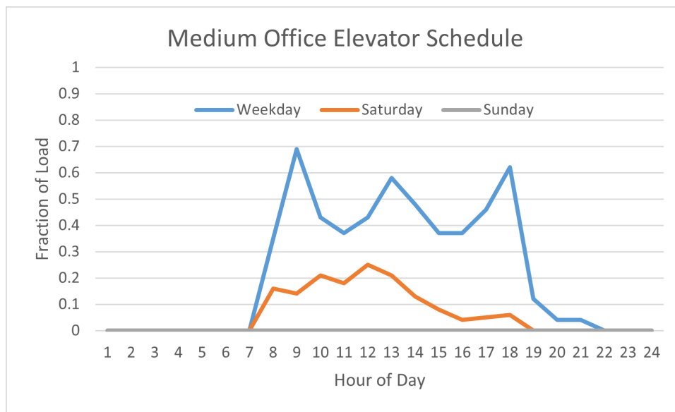
Figure 31. Elevator fractional load schedule for medium offices on weekdays, Saturdays, and Sundays.
