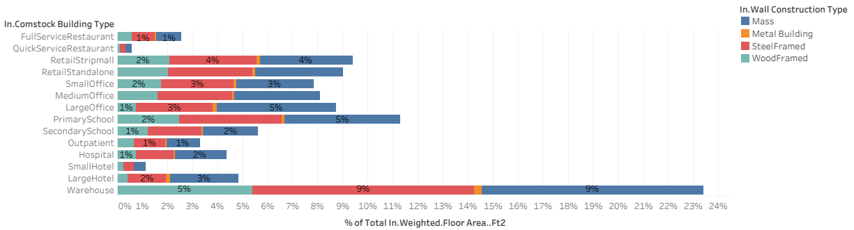
Figure 21. Weighted floor area by wall type and building type.
