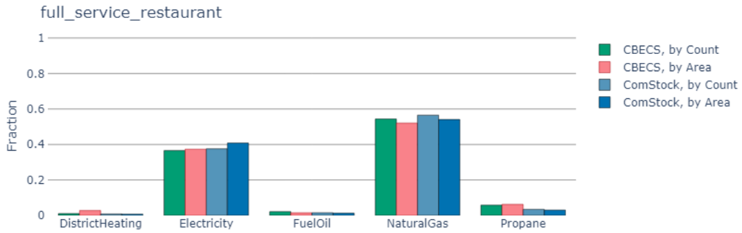
Figure 62. Area-weighted vs. building-count-weighted comparison of fuel type prevalence between ComStock and CBECS for full service restaurants. From left to right, the fuel types on the x-axis are: district heating, electricity, fuel oil, natural gas, and propane.
