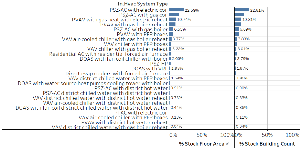
Figure 80. Prevalence of ComStock HVAC system types by total stock floor area and building count; medium offices.
