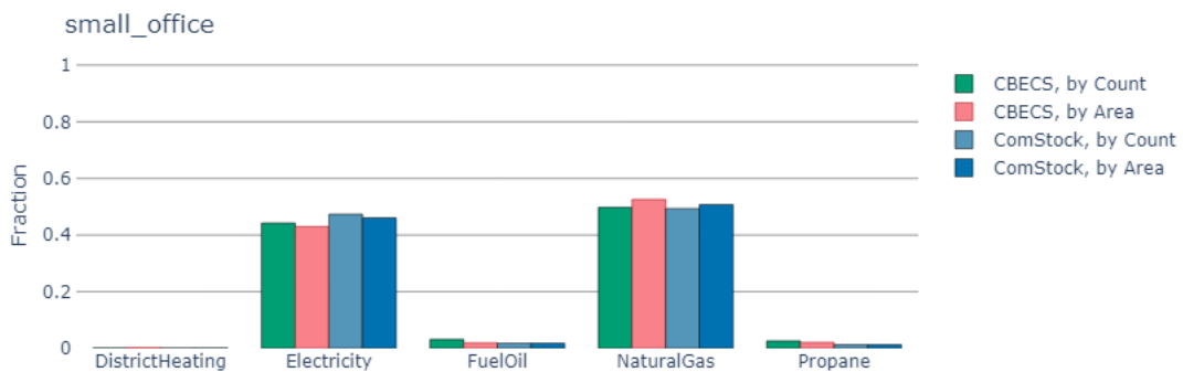
Figure 73. Area-weighted vs. building-count-weighted comparison of fuel type prevalence between ComStock and CBECS for small office. From left to right, the fuel types on the x-axis are: district heating, electricity, fuel oil, natural gas, and propane.
