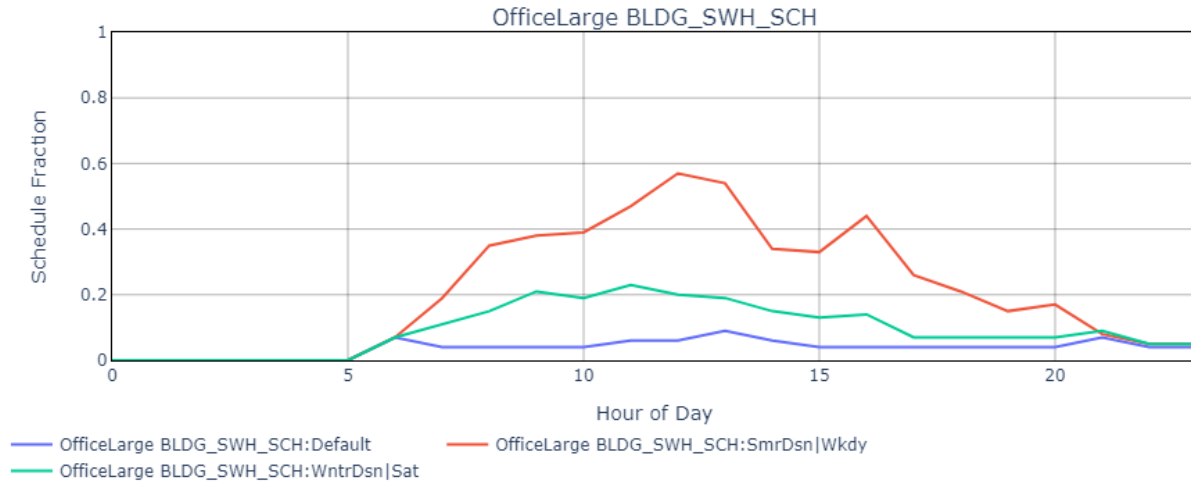
Figure 52. SWH heating usage schedule for large office.
