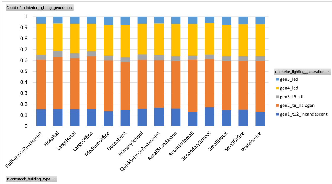
Figure 28. Fraction of installed lighting generation by building type (count-based distribution).
