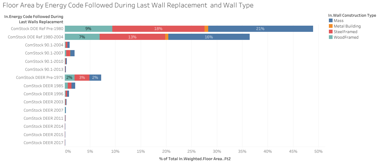
Figure 20. Weighted floor area by energy code followed during last wall replacement and wall type.
