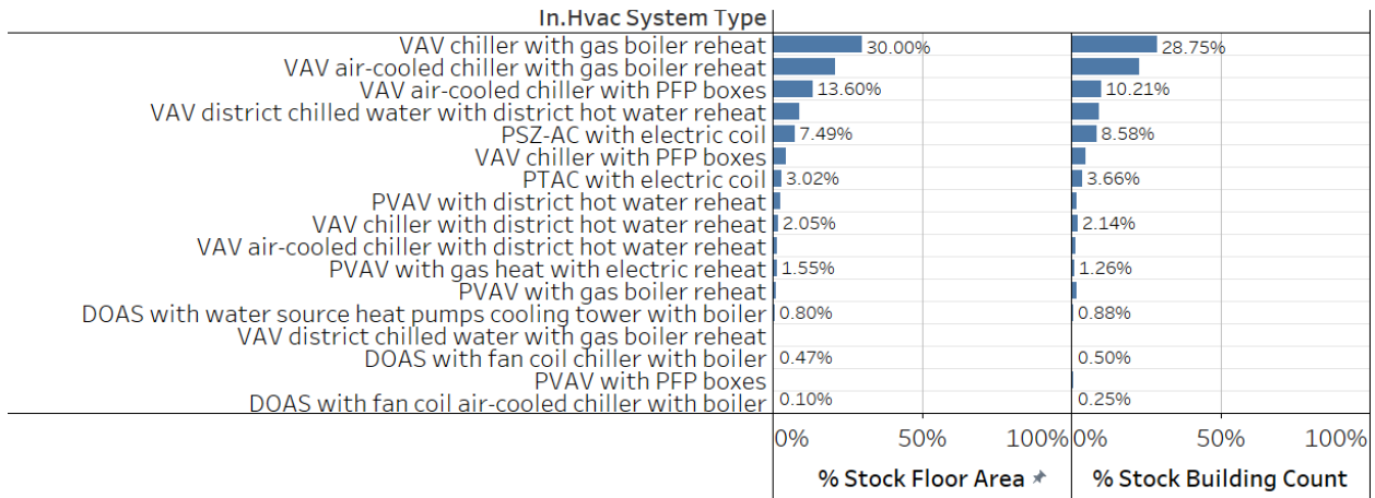
Figure 78. Prevalence of ComStock HVAC system types by total stock floor area and building count; hospitals.
