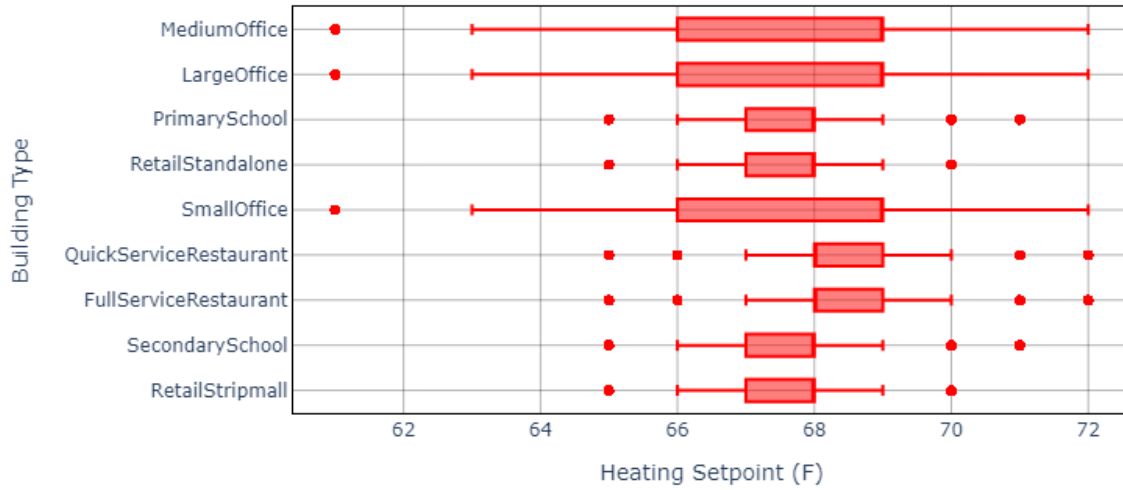
Figure 39. Heating thermostat set point (Fahrenheit) distributions per building type.
